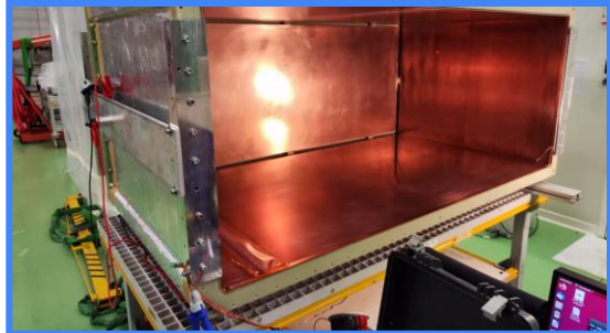
Field Cage + Cathode assembly and test
